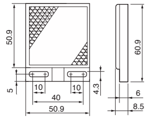
Standard reflector V-61 (Standard, LED type)
