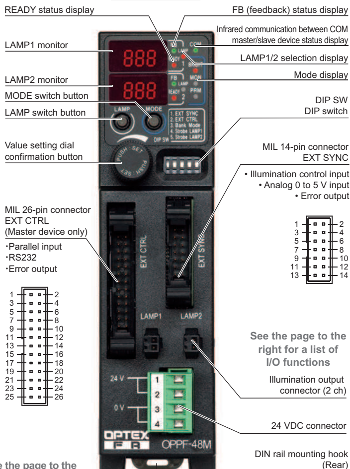
OPPF-48M□ Master device
