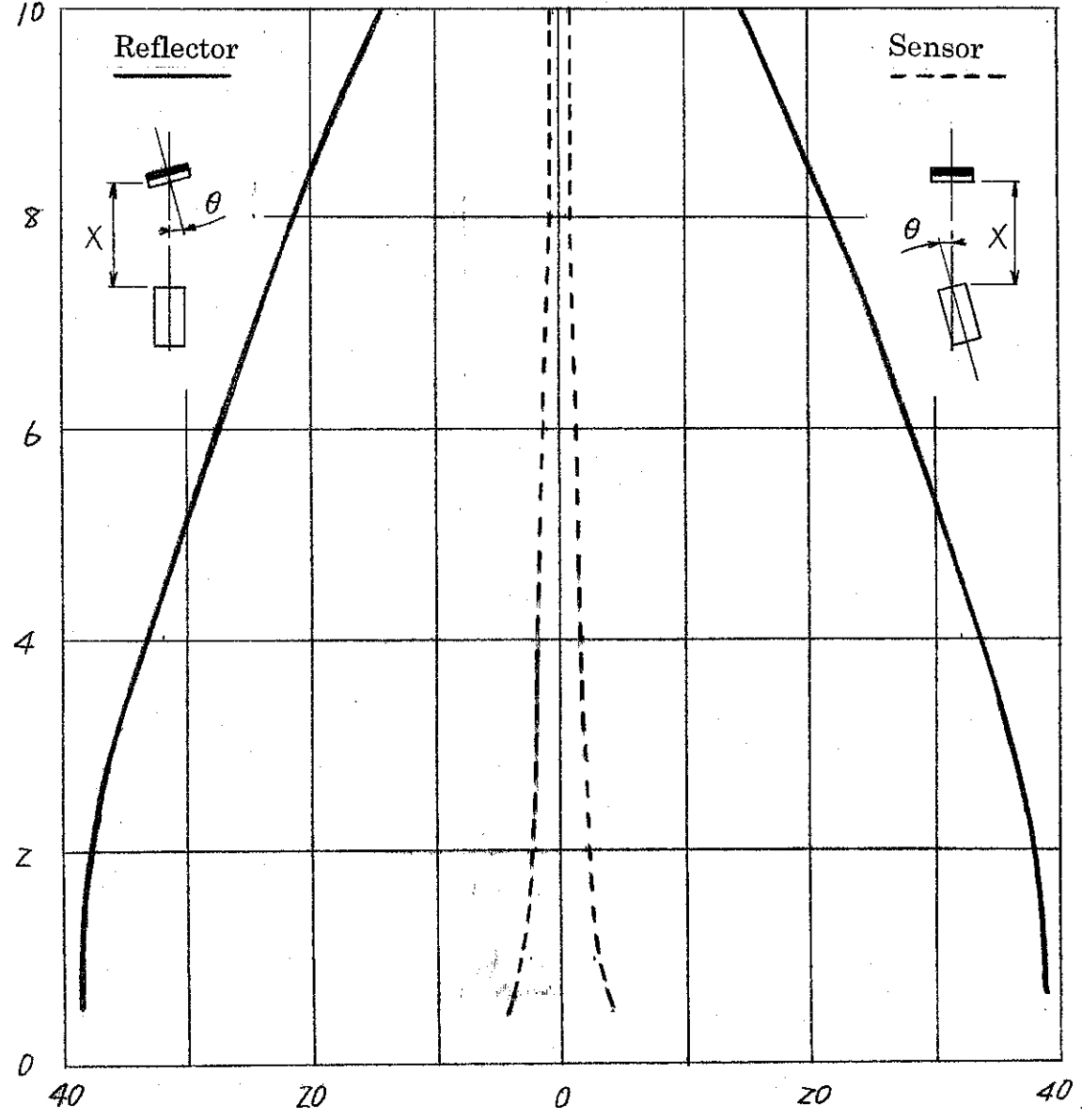
Angle disaligned
