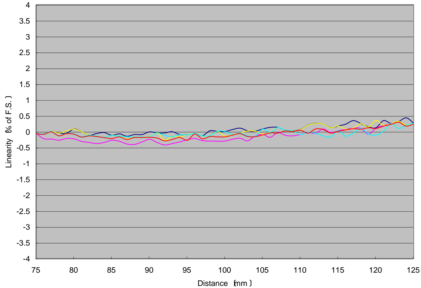
SHP-100 Linearity data ( \pm 5^\circ ) (Typical)
